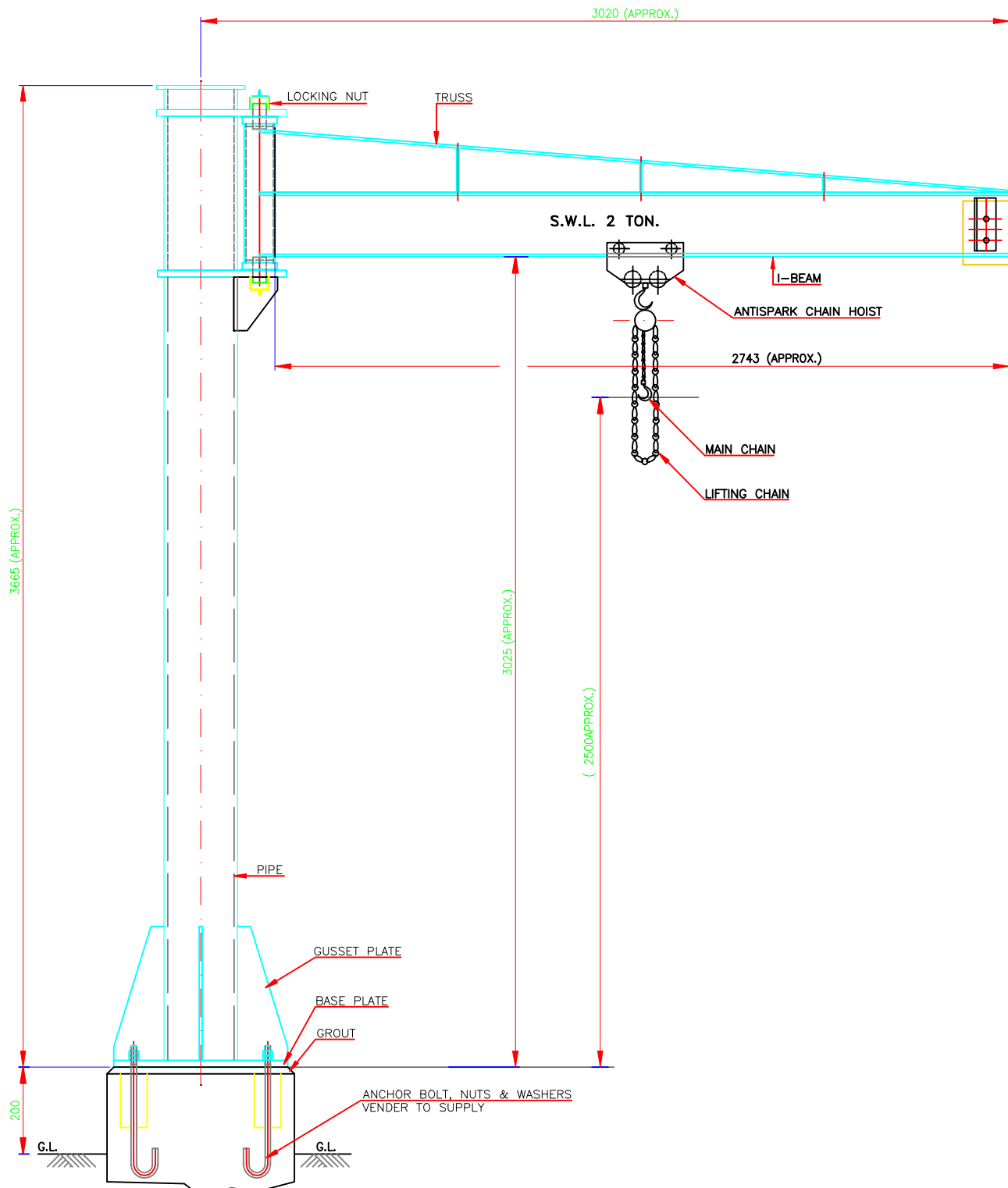
ELEVATION OF JIB CRANE SCALE 1:15
