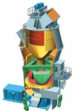
Pfeiffer MPS
