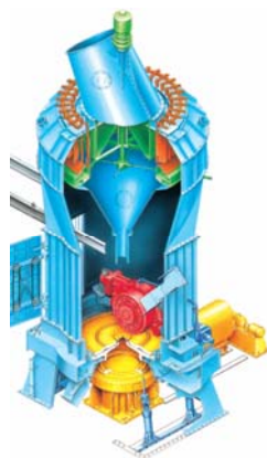
Polysius RM
