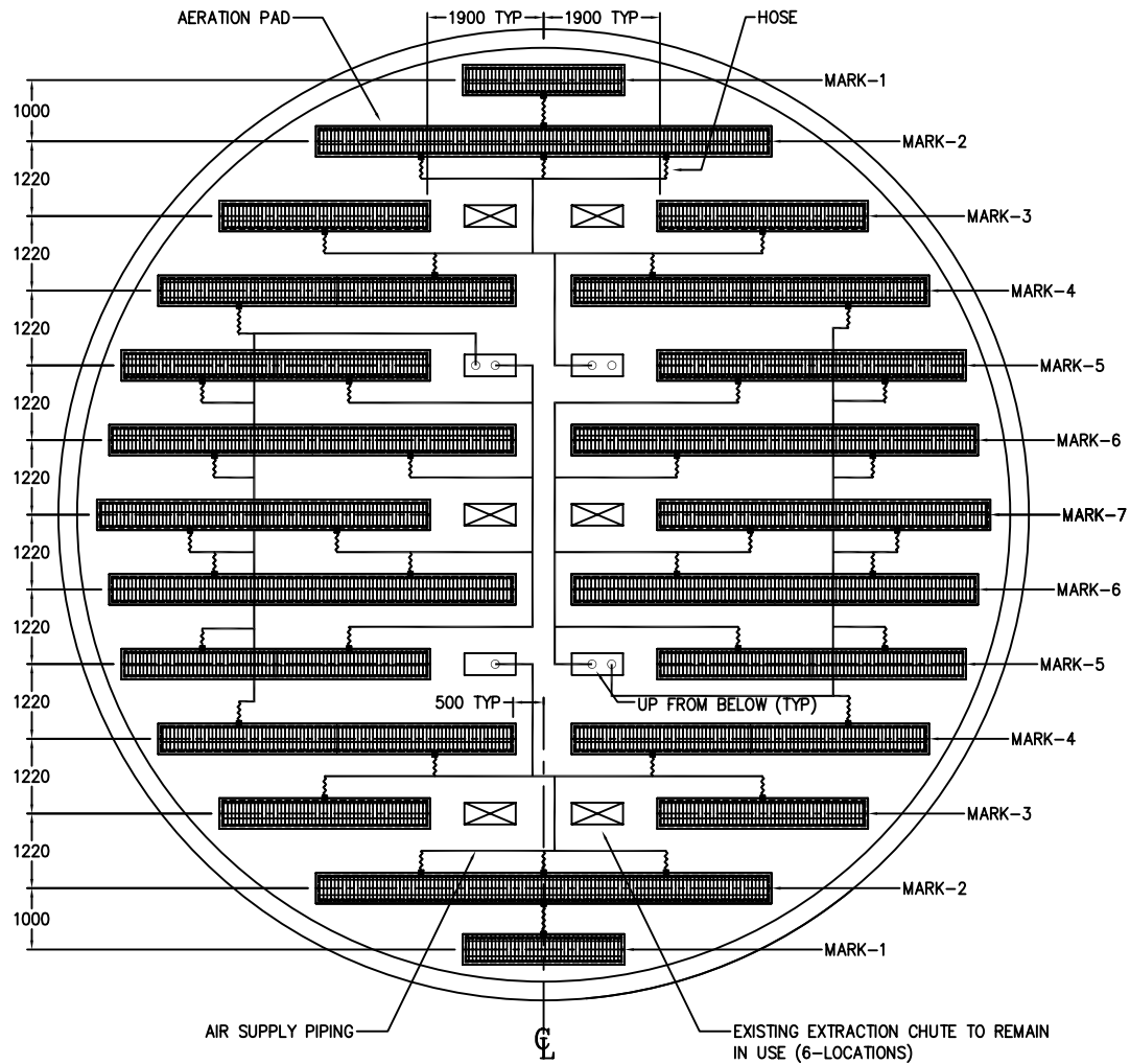
LAYOUT OF AERATION PADS & SUPPLY AIR PIPING
