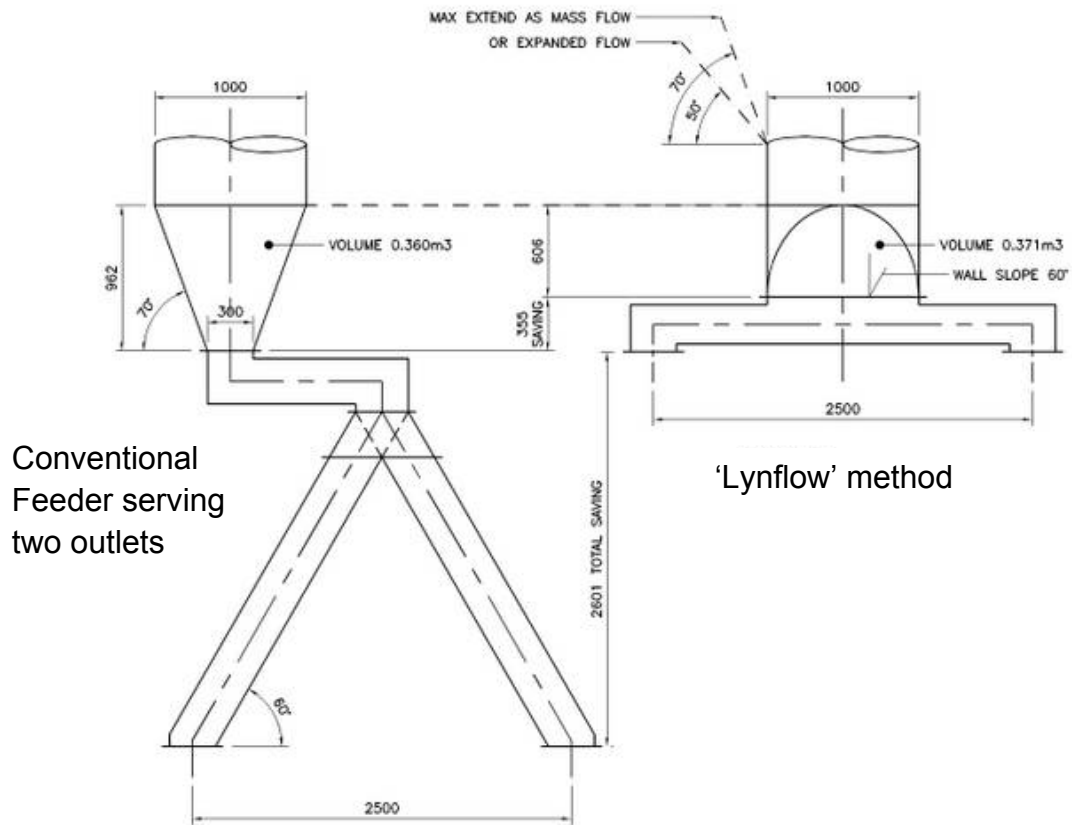
Comparison of 'Lynflow' reversing feeder with conventional method
