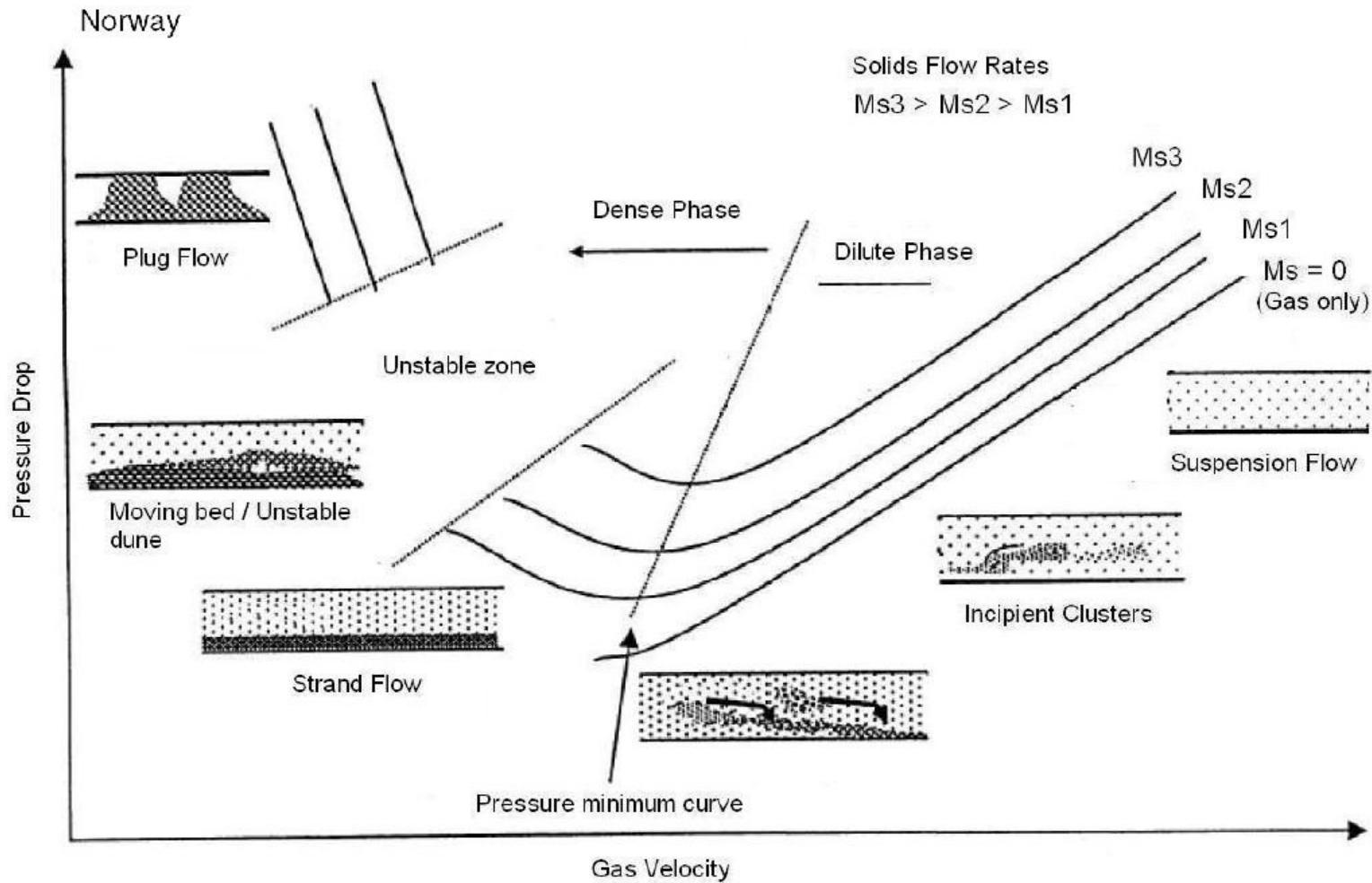
Figure 1-8: A typical conveying characteristic curves: horizontal flow.
