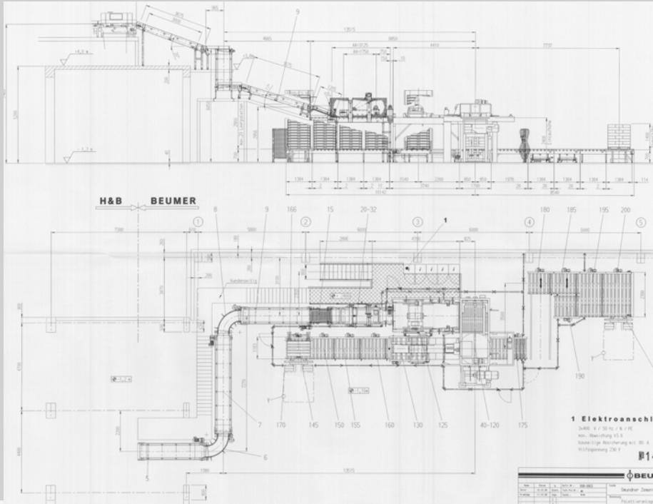
Picture: 2 Paletizing arrangement
