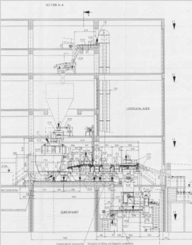
Picture: 3 Rotopacker arrangement
